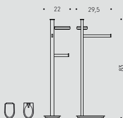
B9113D - B9113S Piantana (Base 24x14 cm) con porta sapone, porta salvietta e porta rotolo Floor standing column with soap holder, towel holder and paper holder
