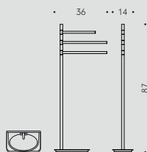
B9915 Piantana (Base 24x14 cm) con 3 porta salvietta Floor standing column with 3 towel holders
