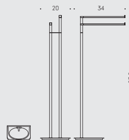
B5038 Piantana (Base 20x20 cm) con due porta salvietta Standing column equipped with two towel holders
