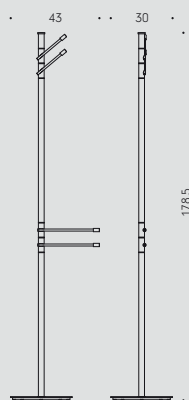
B9412N Piantana con 2 porta salvietta e 2 appendiabiti Floor standing column with 2 towel holders and 2 hooks
