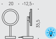
B9750 Specchio ingranditore (3x) da appoggio con luce a LED (220V) incorporata Standing magnifying mirror (3 times) with LED built-in light
