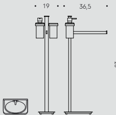
B9111 Piantana (Base 24x14 cm) con spandisapone (L 0,28) porta bicchiere e porta salvietta Floor standing column with soap dispenser, glass holder and towel holder
