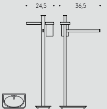
B9110 Piantana (Base 24x14 cm) con porta sapone, porta bicchiere e porta salvietta Floor standing column with soap holder, glass holder and towel holders
