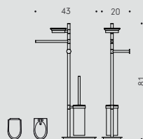
B9903 Piantana (Base 24x14 cm) con porta salvietta, porta sapone, porta rotolo e porta scopino sospeso in vetro acidato Floor standing column with towel holder, soap holder, paper holder and suspended acid glass brush holder
