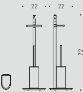
B9807 Piantana (Base 22 cm) con porta rotolo e porta scopino in ottone Floor standing column with paper holder and brass brush holder
