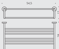
B2787 Rack porta salvietta Rack towel holder
