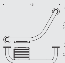
B9722 Maniglione da vasca con porta sapone reversibile Bath grab-bar with reversible soap shelf complies with UNI 11064:2003
