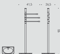
B9415N Piantana (Base 26,5 cm) con 3 porta salvietta Floor standing column with 3 towel holders
