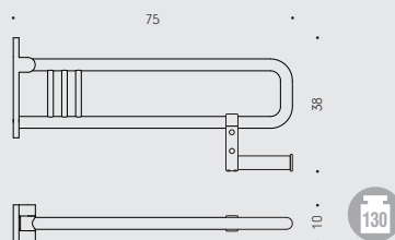
B9730 Appoggio ribaltabile con portarotolo Folding support with paper holder
