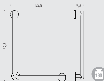
B9732 Sostegno a 90° reversibile Holding handle 90° reversible
