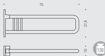
B9728 Appoggio ribaltabile Folding support
