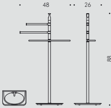
B9803 Piantana (Base 26 cm) con 3 porta salvietta Floor standing column with 3 towel holders
