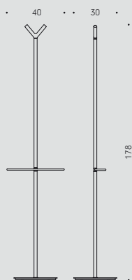
B9804 Piantana (Base 30 cm) con porta salvietta e 2 appendiabiti Floor standing column with towel holder and 2 hooks
