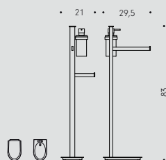
B9119D - B9119S Piantana (Base 24x14 cm) con spandisapone (L 0,28) porta salvietta e porta rotolo Floor standing column with soap dispenser, towel holder and paper holder
