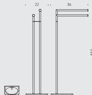
B4038 Piantana (Base Ø22 cm) con due porta salvietta Standing column equipped with two towel holders
