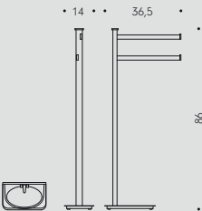
B9103 Piantana (Base 24x14 cm) con 2 porta salvietta Floor standing column with 2 towel holders
