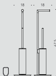
B4018 Piantana (Base Ø18 cm) con porta rotolo e porta scopino Standing column equipped with paper holder and brush holder
